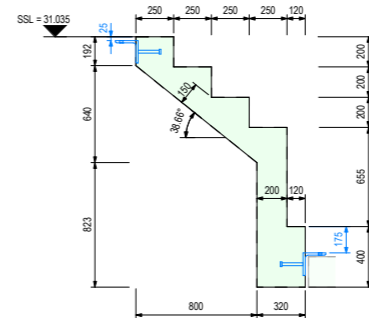
C Section C-C 1:25
