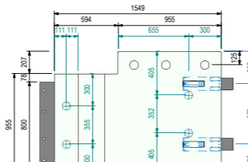
E Section E-E 1:25
