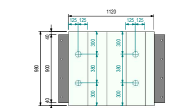
C Section C-C 1:25
