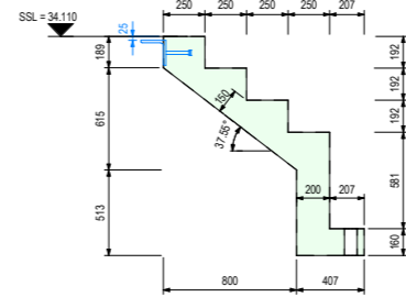
F Section F-F 1:25
