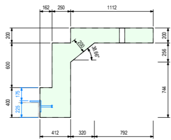
B Section B-B 1:25
