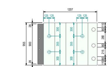
F Section F-F 1:25
